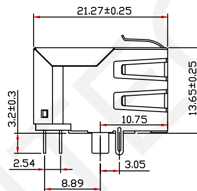
with EMI Shield
